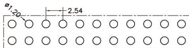
P. C. B LAYOUT
