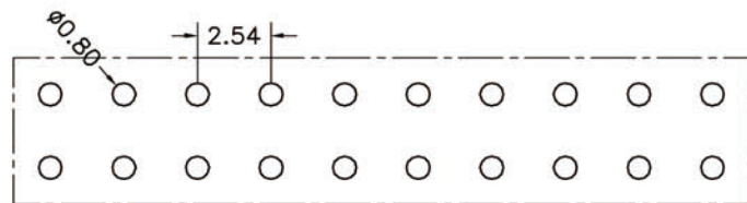
P. C. B LAYOUT
